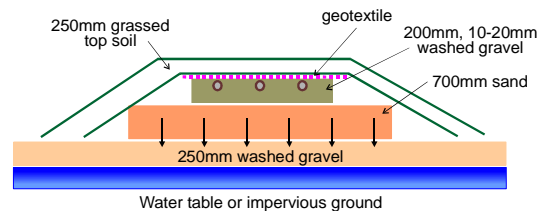
Typical Drainage Mound
